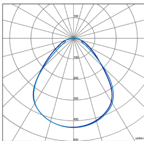
PSB/MCR-UGR<18-38W
